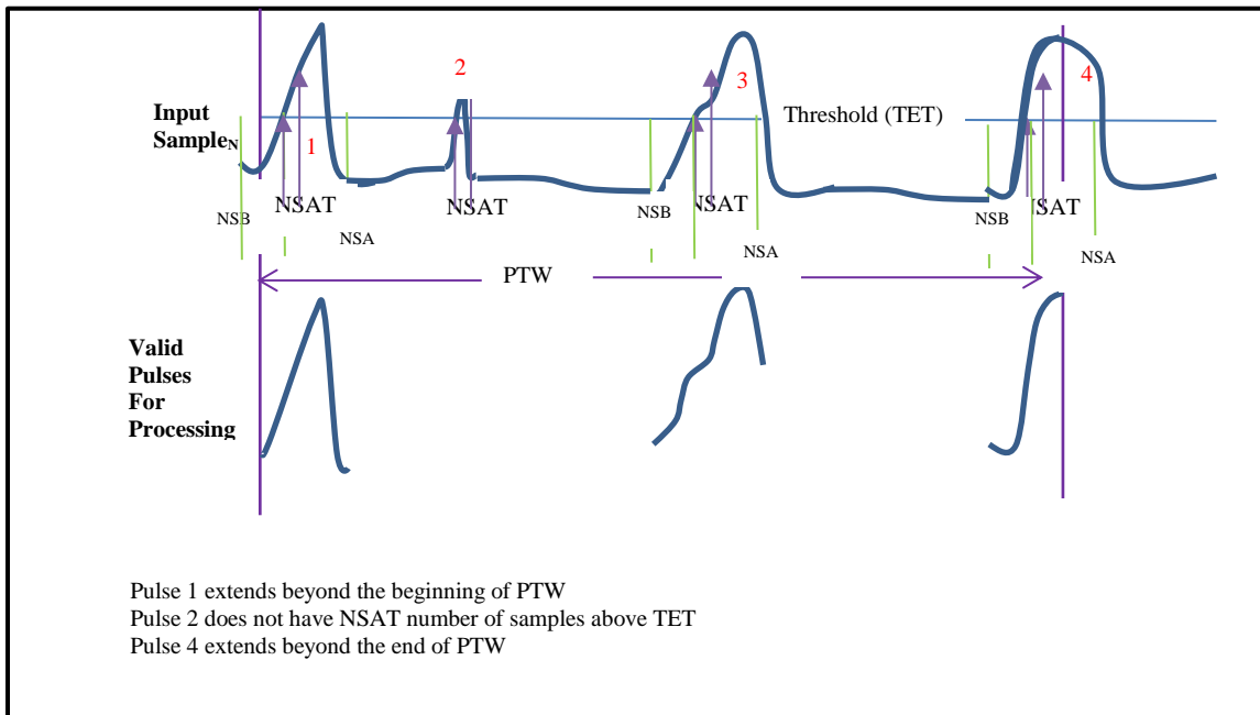
Figure 2 : Pulse Definition
