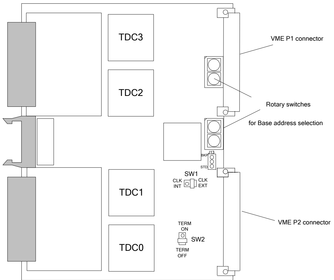
Fig. 3.5: Component Location (V1190 A 5 )
