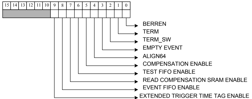
Fig. 6.9: Control Register
