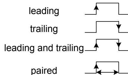
Fig. 2.2: Pulse detection
